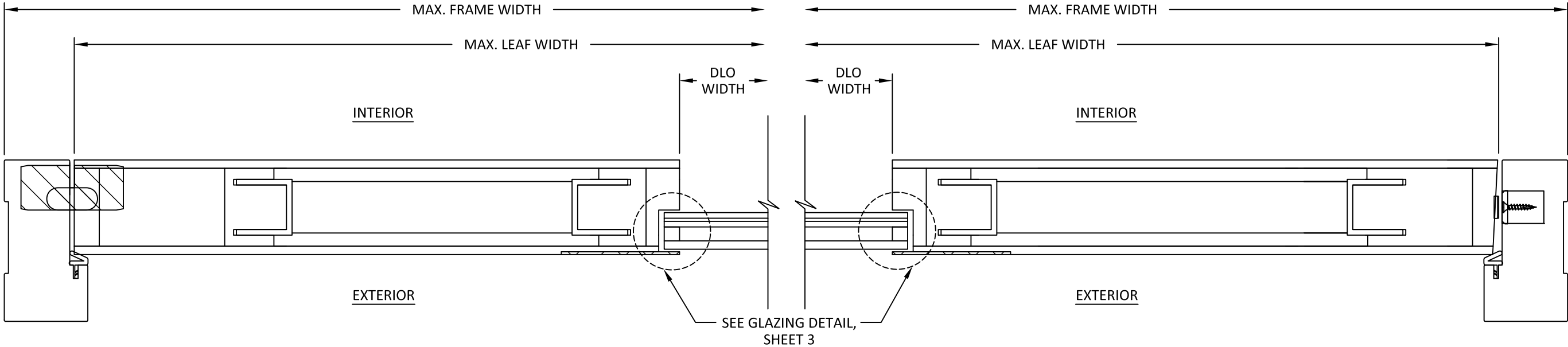
C 5 HORIZONTAL SECTION HINGE JAMB - CONCEALED HINGE FRAME
