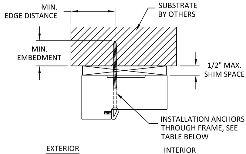
F 6 VERTICAL SECTION HEAD - CONCEALED HINGE FRAME
