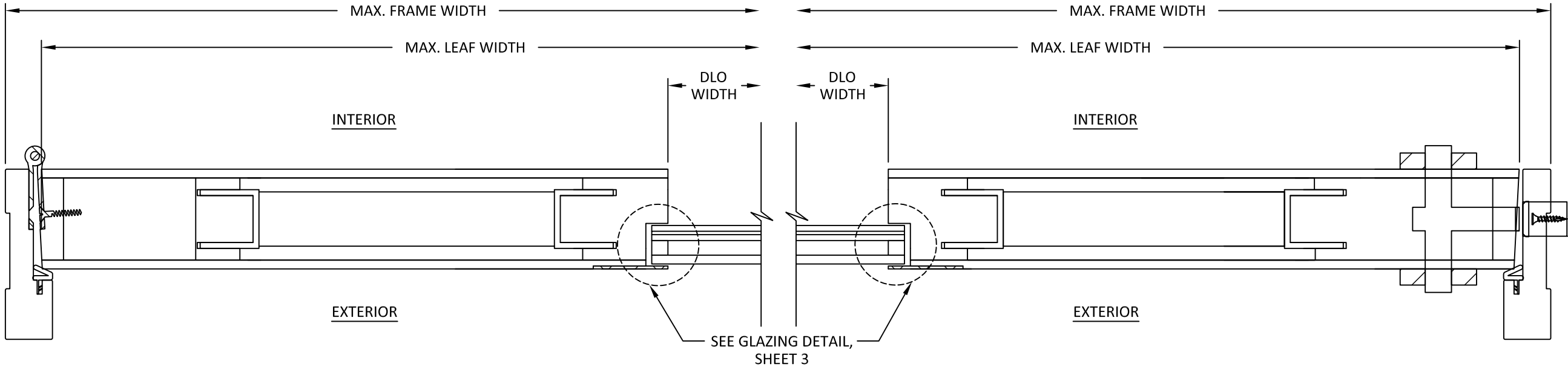
A 5 HORIZONTAL SECTION HINGE JAMB - BUTT HINGE FRAME
