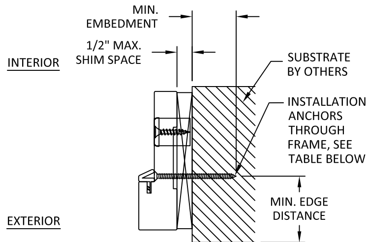
B 6 HORIZONTAL SECTION LOCK JAMB - BUTT HINGE FRAME
