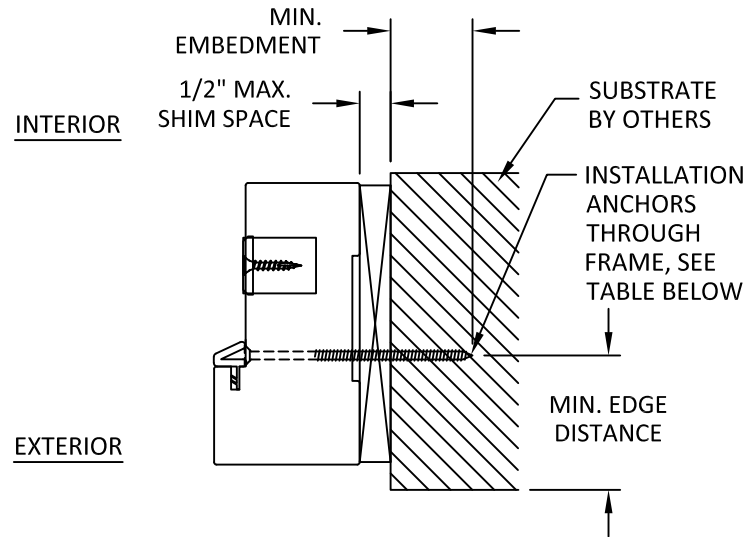
E 6 HORIZONTAL SECTION LOCK JAMB - CONCEALED HINGE FRAME
