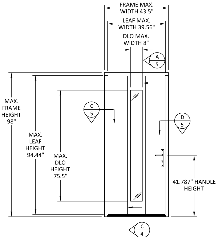
ELEVATION CONCEALED HINGE FRAME
