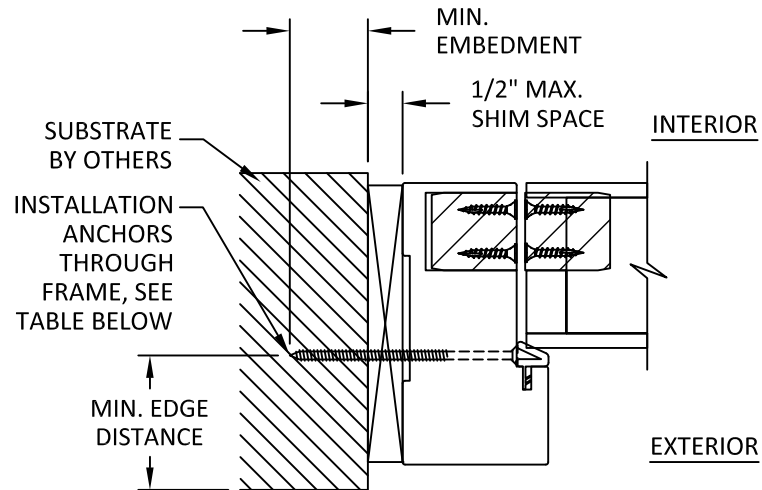
A 6 HORIZONTAL SECTION HINGE JAMB - BUTT HINGE FRAME
